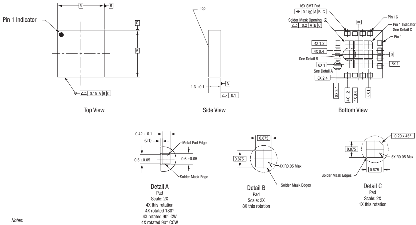
Figure 26. SKY66289-11 Package Dimensions
